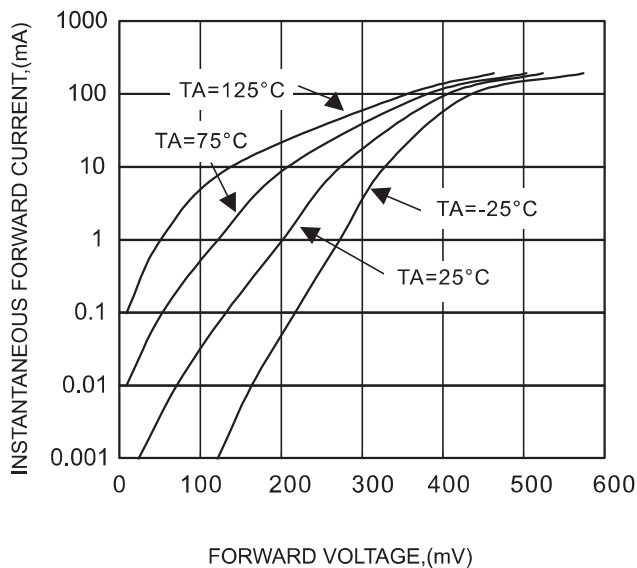
FIG.1-TYPICAL FORWARD CHARACTERISTICS
